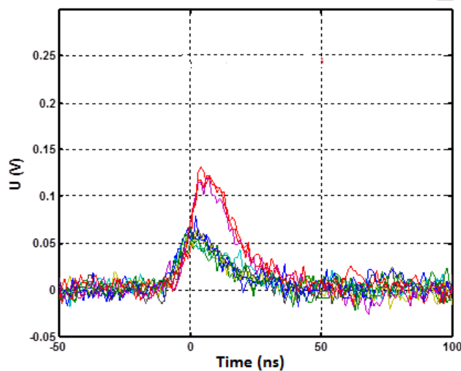
Fig. 8. PD-induced pulses obtained with HTFC B.
