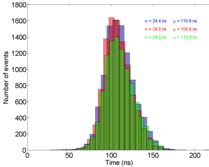
Fig. 13. FWHM distribution of neutron-induced pulses obtained with HTFC B at 200°C (blue), 400°C (red) and 600°C (green).
