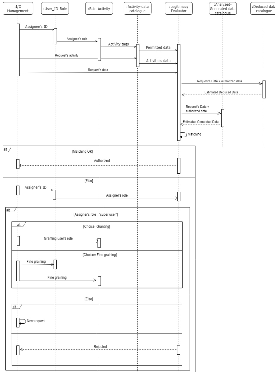
Fig. 2. Data access legitimacy evaluation's sequence diagram
