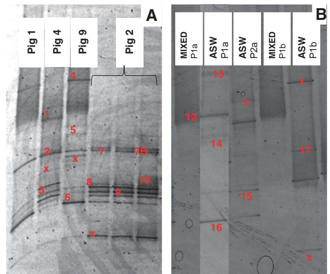
Fig. 10. DGGE gel profile demonstrating diversity of bacterial populations based on PCR products of 550 bp of bacterial 16S rRNA. (A) Profile obtained using directly the pigging debris as samples (Fig 2 in triplicate) (sequenced bands were labelled 1-11; not yield results were labelled "x"), and (B) profile obtained from cultivable bacteria that grew in ASW supplemented and MIXED water supplemented used to perform the electrochemical experiments (bands sequenced labelled 12-30).
