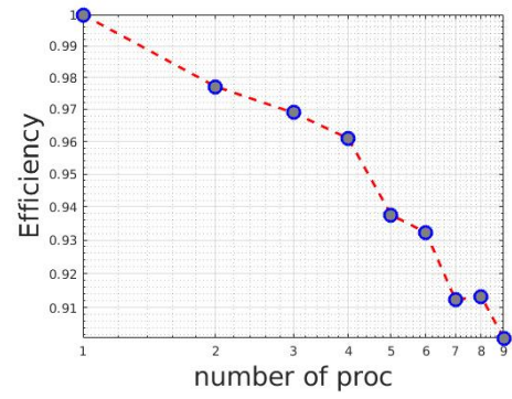
Figure 3: The 2D homogeneous heat equation. Speedup (left) and Efficiency (right) as a function of the number of processors.
