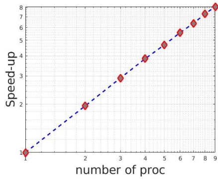
Figure 3: The 2D homogeneous heat equation. Speedup (left) and Efficiency (right) as a function of the number of processors.
