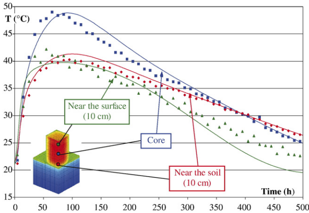
Fig. 4. Temperature variations for different points of concrete block: comparison between experiment (points) and model (curves).
