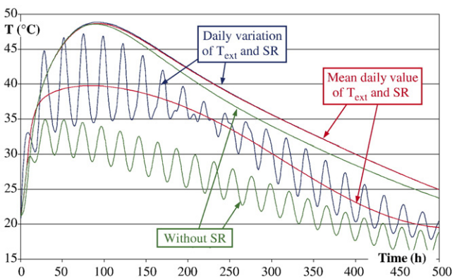
Fig. 5. Temperature variation in concrete block for different ambient conditions ( T_{ext} : ambient temperature, SR: solar radiation) (for the color convention see Fig. 4) (For interpretation of the references to color in this figure legend, the reader is referred to the web version of this article.)
