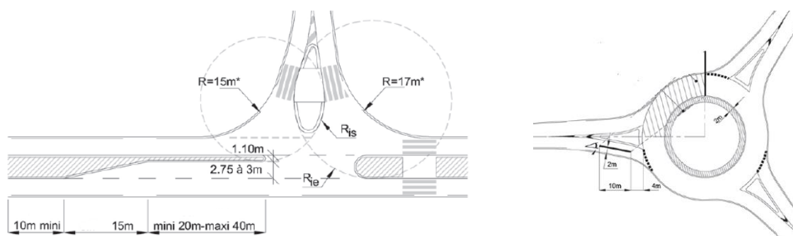
Figure 3: Example of the geometrical characteristics of an intersection (left) and Nominal roundabout (right; the radius of the outer ring should be between 15 and 25 m), from [4].
