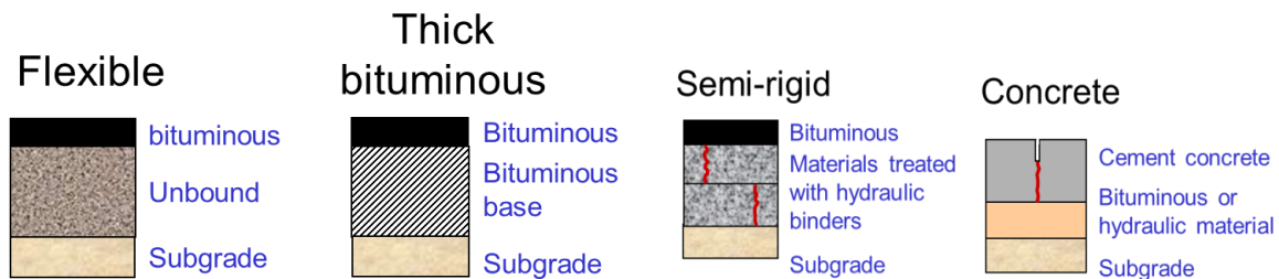
Figure 1: Typical pavement structures.
