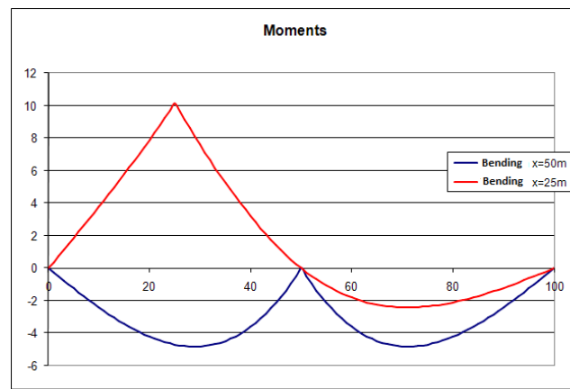
Figure 2: Bending moment at midspan ((red curve) and on support (blue curve), for two-span structure with both span lengths equal to 50 m.
