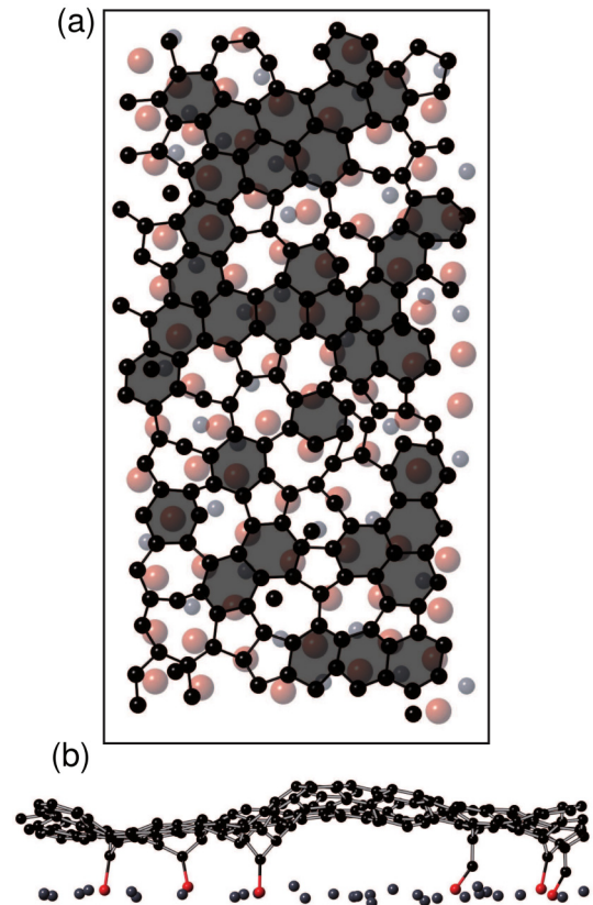
FIG. 6. Equilibrium structures at 700 K, obtained from GCMC simulations performed on a Ni 2 C/Ni(111) interface for \mu_C = -5.15 eV/atom. Ni atoms are orange, C atoms of Ni 2 C are gray, and outer C atoms on the surface to form graphene are black. The Ni atoms from Ni(111) are omitted for clarity. (a) Top view, where many hexagons can be seen. (b) Side view, where C-C bonds between graphene and the interface (C atoms are in red) are clearly present.
