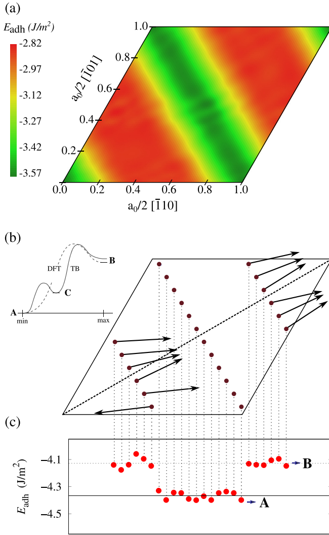
FIG. 2. Relative stability of the \text{Ni}_2\text{C} layer on the \text{Ni}(111) substrate, with the TB model. (a) Map of adhesion energies, as computed with Eq. (1), for all possible shift vectors \vec{F} and with atomic relaxations performed only along the \text{Ni} [111] direction. (b) Scheme showing the \vec{F} vectors of the specific configurations of the \text{Ni}_2\text{C}/\text{Ni}(111) that are then fully relaxed. The arrows indicate the in-plane displacement experienced by the \text{Ni}_2\text{C} layer relative to the \text{Ni}(111) substrate during a subsequent annealing of the structures (see text). The inset illustrates the aspect of the energy landscape along the [211] direction for TB and DFT. (c) Fully relaxed adhesion energies for these selected configurations.
