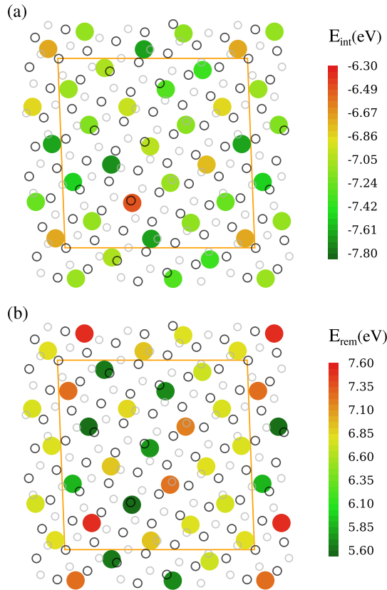
FIG. 3. Maps representing (a) the interaction energies [Eq. (2)] of a single C atom forming a C dimer with the Ni 2 C/Ni(111) system and (b) the energy cost to remove a C atom from the carbide layer [Eq. (2)]. Energies are computed for all C atom positions in the Ni 2 C layer within the supercell, adopting the following representation: big dots correspond to C atoms from Ni 2 C and are colored according to the appropriate energy value, and open circles represent two successive (111) layers of fcc Ni. Atomic positions are from the relaxed initial group-A configuration before adding or removing carbon. The Ni atoms from the carbide are omitted for clarity.
