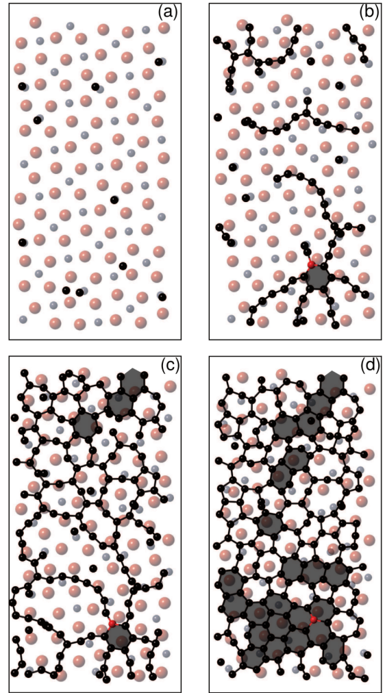
FIG. 5. Snapshots of atomic configurations during the growth of graphene on a \text{Ni}_2\text{C}/\text{Ni}(111) interface at 500 K and \mu_C = -4.75 eV/atom. Ni atoms are orange, C atoms of \text{Ni}_2\text{C} are gray, and outer C atoms on the surface to form graphene are black. The Ni atoms from \text{Ni}(111) are omitted for clarity. (a) Atoms adsorbed on top of C atoms of \text{Ni}_2\text{C} . (b) C atoms of the interface (in red) integrated into the graphene network. (c) Chains forming and crossing to form hexagons. (d) Equilibrium structures at 500 K.
