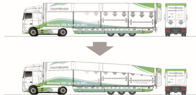
Fig. 4 Load Optimisation Combination with Double Floor Loading System and Aerodynamic Measures (adjustable roof, boat tail, side skirts)
