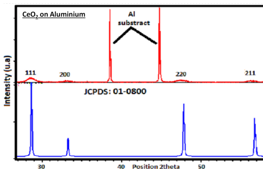
Figure 1: XRD patterns of the cerium oxide films elaborated at current density of 5 mA cm -1 for 120 min in 0.1 M Ce(NO 3 ) 3 is in agreement with the JCPDS card no 01-0800.
