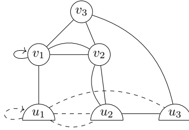
Figure 4.1: Example of a graph in \mathbf{VGr}_m (for m \geq 2 )
