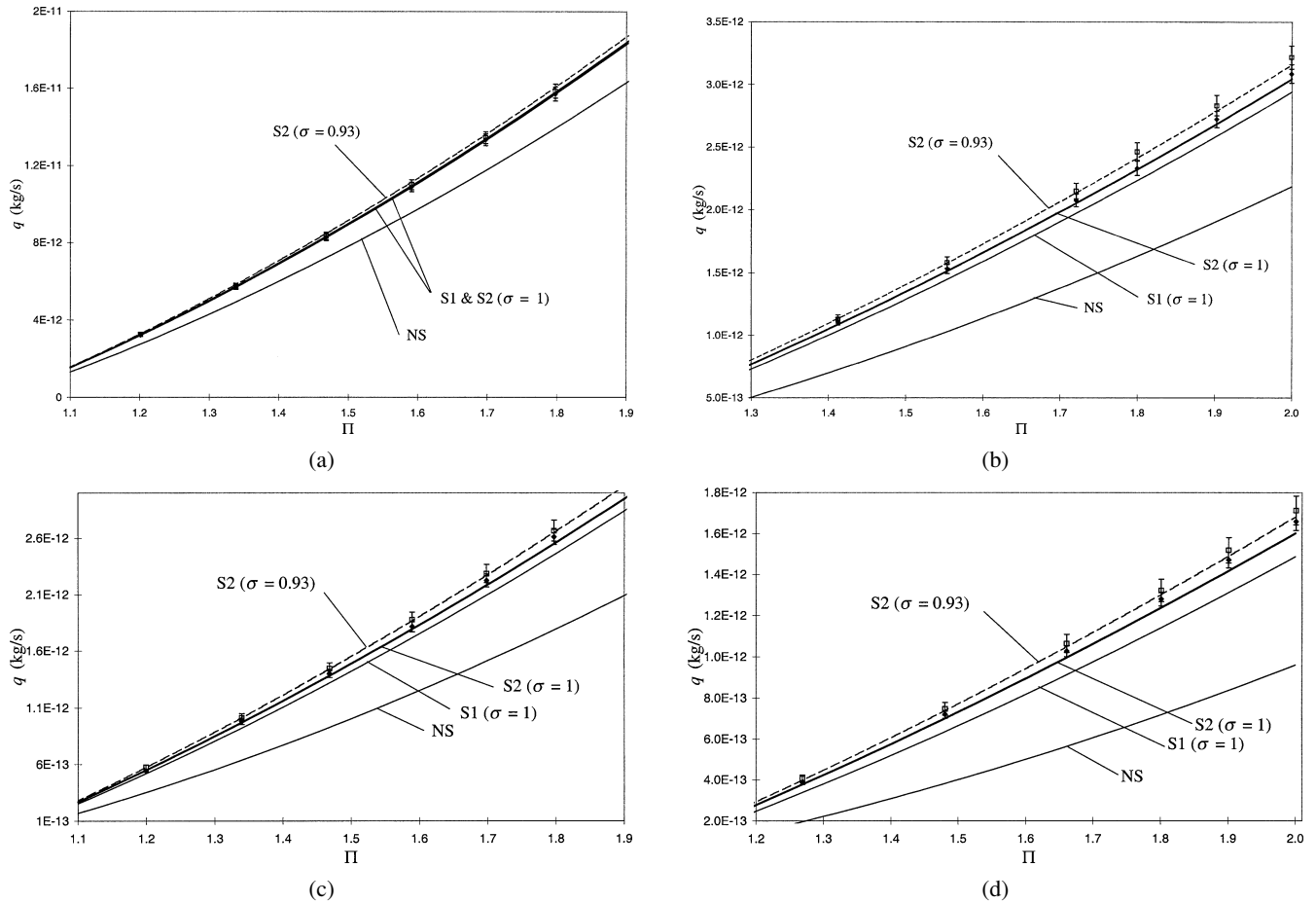
Figure 7 Theoretical and experimental mass flow rates. Wafer n o 3, 2h = 1.16 \mu\text{m} , T = 294.2 \text{ K} . a) gas: \text{N}_2 , 0.016 \leq \text{Kn}_o \leq 0.03 , P_o = 1.9 \cdot 10^5 \text{ Pa} ; b) gas: \text{N}_2 , 0.04 \leq \text{Kn}_o \leq 0.09 , P_o = 0.65 \cdot 10^5 \text{ Pa} ; c) gas: \text{He} , 0.05 \leq \text{Kn}_o \leq 0.09 , P_o = 1.9 \cdot 10^5 \text{ Pa} ; d) gas: \text{He} , 0.1 \leq \text{Kn}_o \leq 0.22 , P_o = 0.75 \cdot 10^5 \text{ Pa} .
