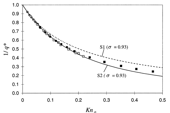
Figure 8 Inverse reduced flow rate ( 1/q^* ) in rectangular microchannels. Comparison of experimental data with 1st and 2nd order slip flow models. \Pi = 1, 8 ; T = 294, 2 \text{ K} . Wafer n o 2 (white), n o 3 (grey), n o 4 (black). Gas: \text{N}_2 (circle) and \text{He} (square).
