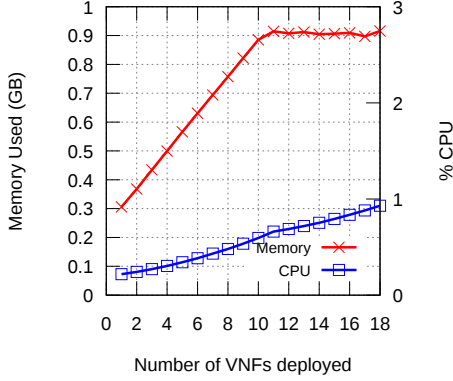
Fig. 5: RAM and CPU used as a function of the number of deployed Apache 2 with PHP module VNF.
