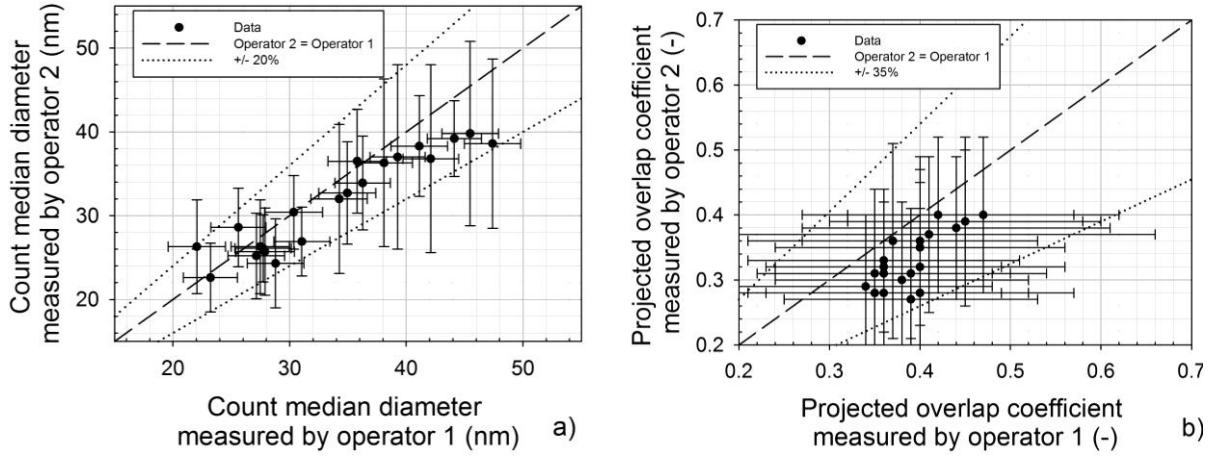
Figure 1: Comparison between count median primary spheres diameters (a) and projected overlap coefficients (b) measured by two human operators for soot particles produced by an ethylene diffusion flame (adapted from Ouf et al., 2010). Bars represent standard deviations.
