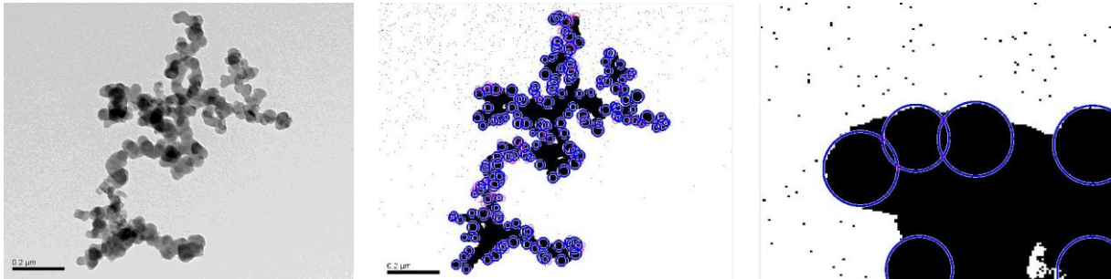
Figure 3: Illustration of the primary particle diameter and overlap coefficient measurement process
