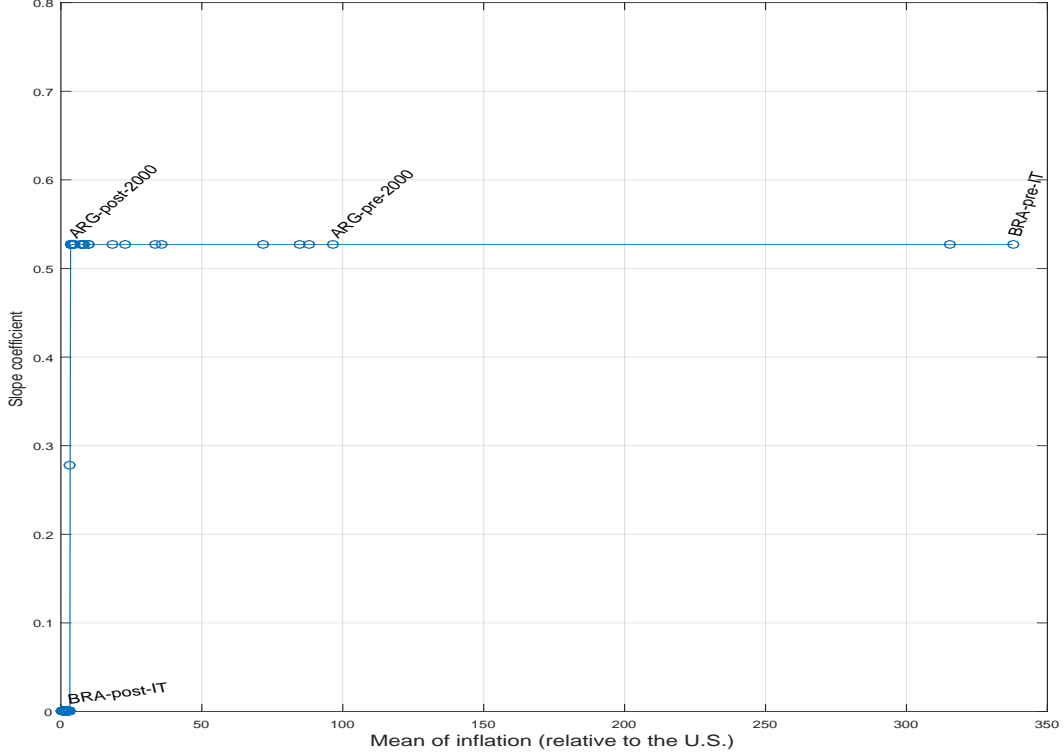
Figure 2: Slope coefficients estimated by PSTR model
