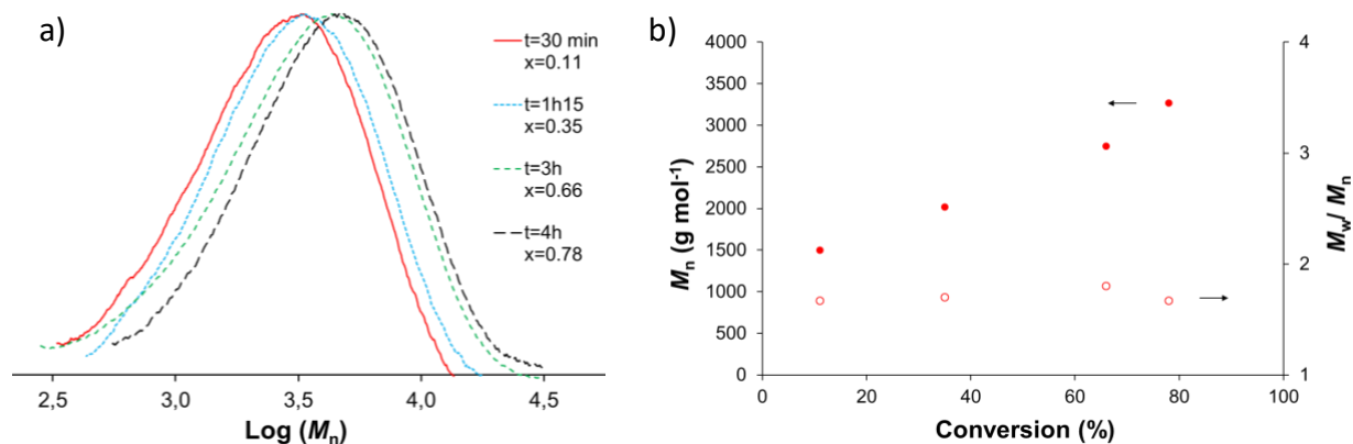
Figure 3. Synthesis of PNAM2 : a) SEC-THF monitoring of the polymerization; b) Experimental M_n and dispersity as a function of monomer conversion (values obtained from conventional calibration against PS standards).
