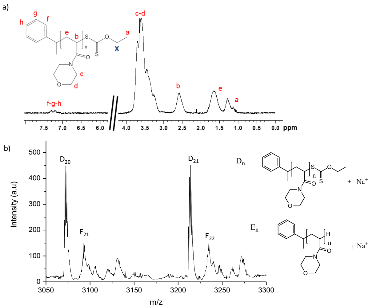
Figure 4. a) 1 H NMR spectrum of PNAM2 (D 2 O) ; b) Enlarged MALDI-ToF mass spectrum of PNAM2 in reflectron mode.
