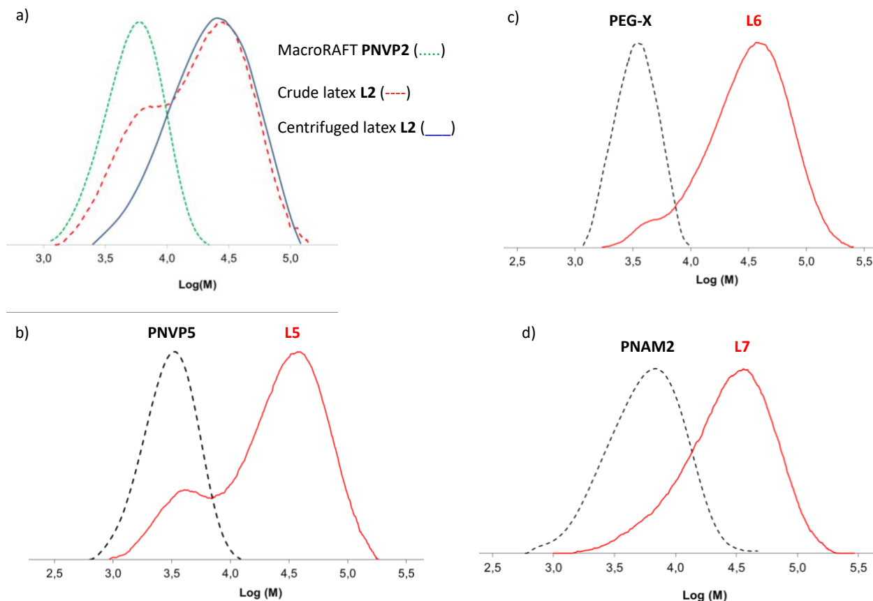
Figure 7. SEC traces in DMF of a) PNVP2 , crude latex L2 , L2 after centrifugation, b) PNVP5 MacroRAFT and crude latex L5 , c) PEG-X MacroRAFT and crude latex L6 and d) PNAM2 MacroRAFT and crude latex L7 .
