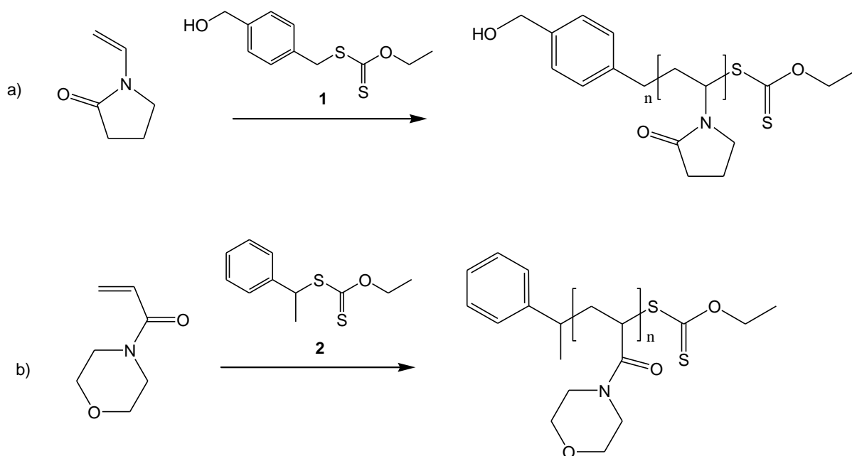
Scheme 1. RAFT/MADIX polymerization of a) N -vinylpyrrolidone (NVP) and b) N -acryloylmorpholine (NAM) using xanthates 1 and 2 , respectively.
