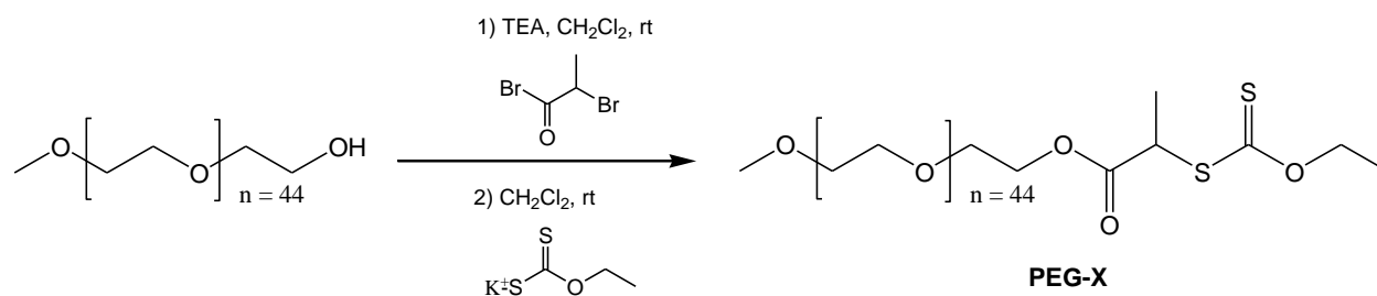
Scheme 2. Synthesis of PEG-X macroRAFT by modification of commercial PEG methyl ether
