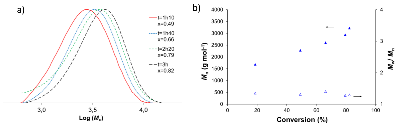
Figure 2. Synthesis of PNVP5 : a) SEC-DMF monitoring of the polymerization; b) Experimental M_n and dispersity as a function of monomer conversion (values obtained from conventional calibration against PMMA standards).
