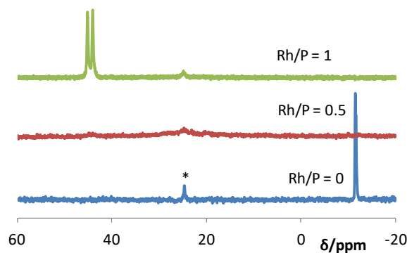
Figure 6. ^{31}\text{P}\{^1\text{H}\} NMR spectra of [\text{Rh}(\text{acac})(\text{CO})(\text{BMOPPP@CCM})] with different amounts of rhodium complex. The starred resonance is due to a minor amount of oxidized phosphine impurity.
