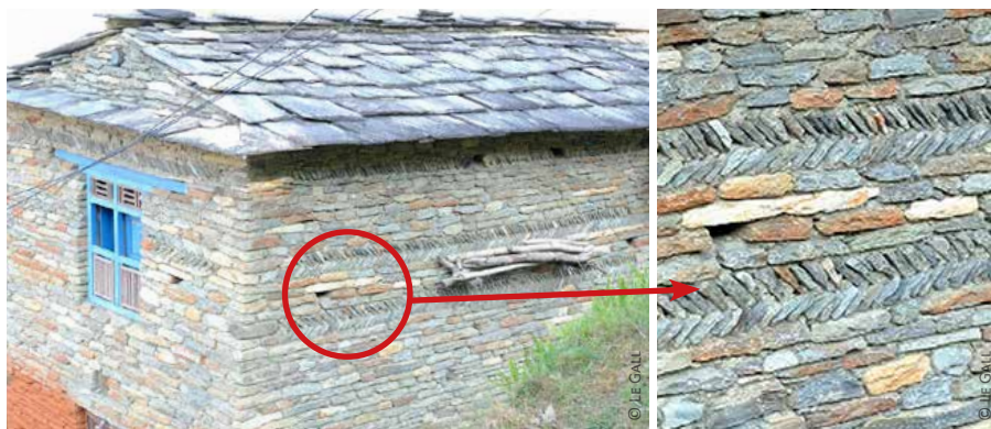
Nepal, after the 2015 M 7.8 Gorkha earthquake: 1) diagonal courses in stone masonry walls with corner stones; 2) opposite directions of layers
