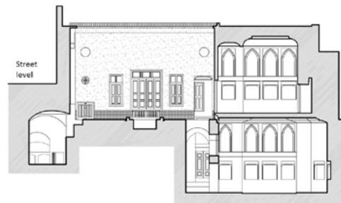
2) Iran: section of a Qajar house in Yazd
