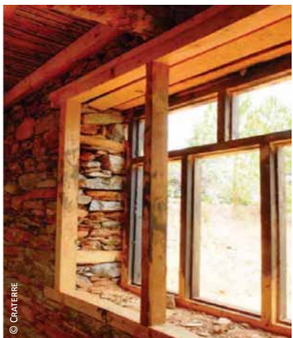
Nepal: 1) a window with a double timber frame; 2) the double frame of a window supporting the roof after the failure of a masonry wall during 2015 Gorkha earthquake
