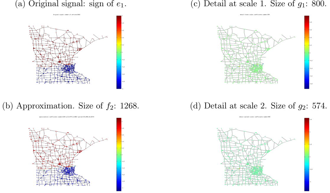
FIGURE 6. Two steps of the intertwining wavelets multiresolution upsampling to the original graph: (a) f_0 ; (b) \bar{R}_0\bar{R}_1f_2 ; (c) \bar{R}_0g_1 ; (d) \bar{R}_0\bar{R}_1g_2
