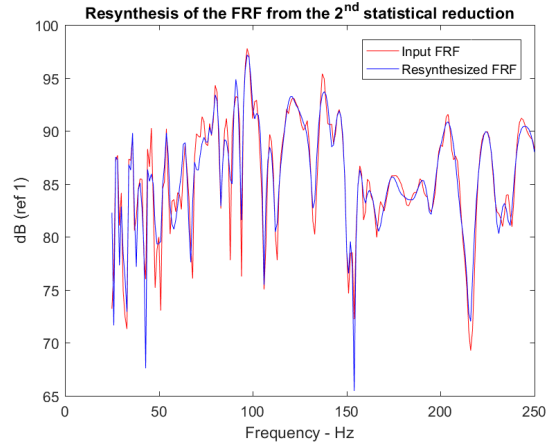
Figure 12: Resynthesized FRF from the second statistical reduction
