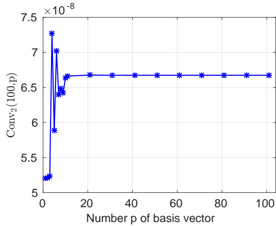
Figure 6: Convergence analysis related to the second nonlinear reduced-order model : graphs of p \mapsto Conv_{2,NONLIN}(m, p) related to the second reduction (thick line, \star marker).
