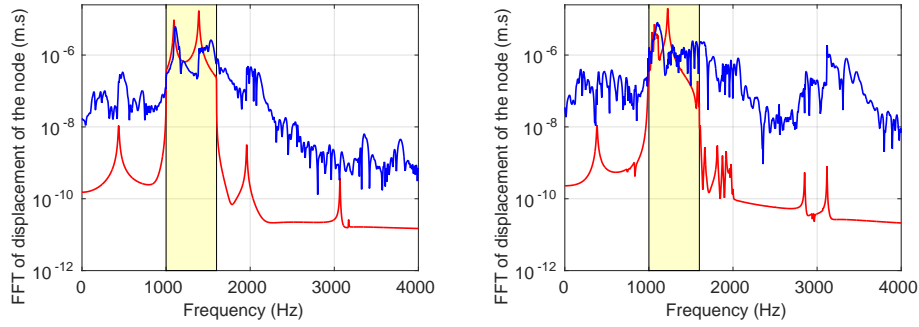
Figure 11: Nonlinear dynamical analysis in the frequency domain: graphs of \nu \mapsto \|\widehat{\mathbf{U}}_{\text{LIN}}^{\text{obs}, j_0}(2\pi\nu)\| (red line) and \nu \mapsto \|\widehat{\mathbf{U}}_{\text{NONLIN}}^{\text{obs}, j_0}(2\pi\nu)\| (blue line) corresponding to patterns \mathcal{P}_1 (left figure) and \mathcal{P}_2 (right figure).
