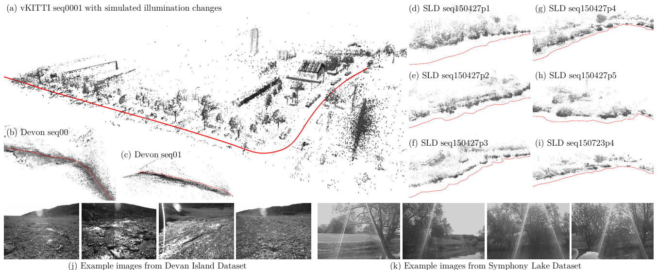
Fig. 4. The qualitative results of tracking and 3D scene reconstruction are presented utilizing synthetic vKITTI Dataset in (a), real-world Devon Island Dataset in (b) (c), and our Symphony Lake Dataset in (d) - (i). The example images from Devon Island Dataset in (j) and Symphony Lake Dataset in (k) are provided, all of which suffer from the global+local illumination changes induced by solar glare.
