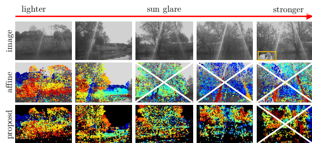
Fig. 5. A collection of images with gradually stronger (left to right) sun glare are chosen to test our system robustness. The reconstructed inverse depth maps using global affine model and our proposed method are presented, where the failure ones are marked with a big 'X'.
