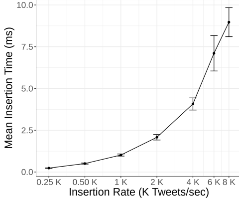
Figure 11: PMQ average insertion time with a window of 6h and varying rates. Current Twitter insertion rate (6K tweets/s) can be processed under 7.5 ms.
