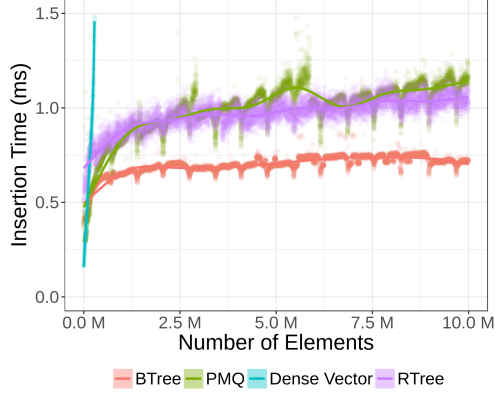
(a) Insertion of 10M elements by batches of 1000 elements.
