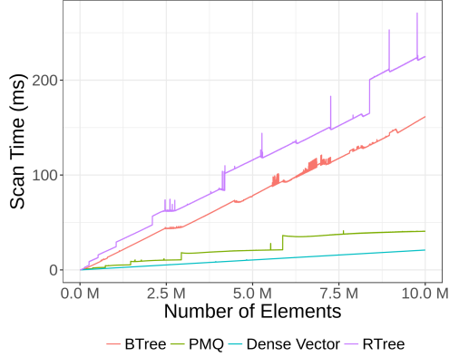
(b) Time for a full scan of the dataset after each batch insertions.
