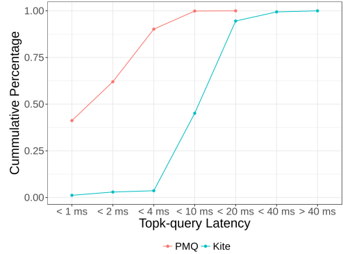
Figure 14: Top-k Queries: cumulative percentages of query latency for K = 100 , R = 30 km and T = 10000 seconds. We compared the search performance of PMQ against the Kite framework.
