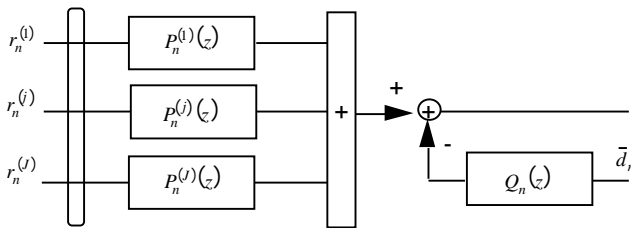
Fig. 3. Multiple-input equalizer
