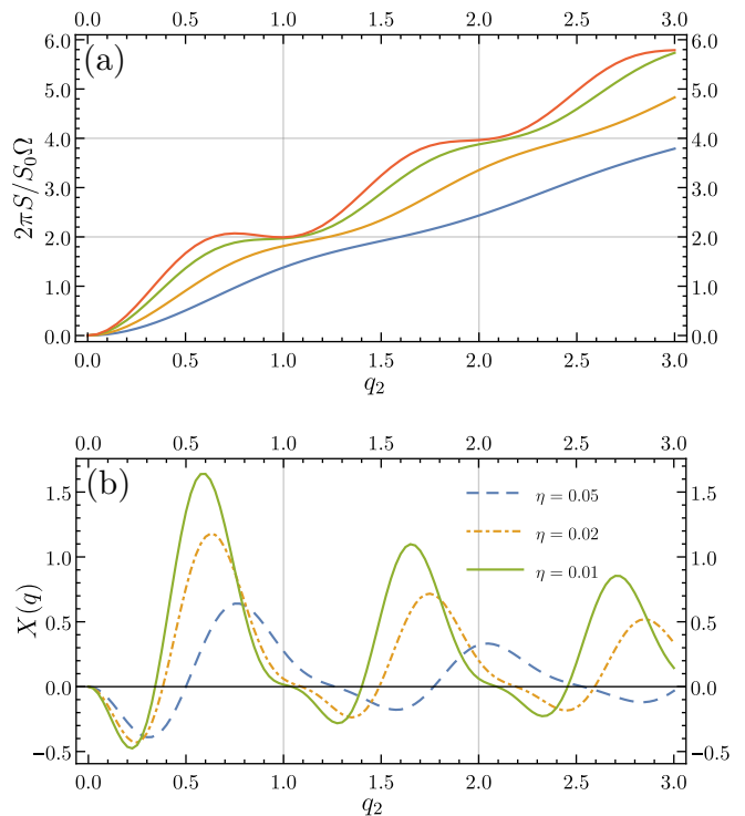
FIG. 6. Panel (a): inner-channel noise 2\pi S/(S_0\Omega) for the periodic Lorentzian drive (44), as a function of q_2 = q\cos\theta\sin\theta , for \tau_d = \mathcal{T}/2 and (from bottom to top) \eta = 0.1, 0.05, 0.02, 0.01 . The value 2q_2 is reached at integer q_2 upon lowering \eta . Panel (b): the function (46) at zero temperature and \tau_d = \mathcal{T}/2 for the Lorentzian drive (44). We note that, upon decreasing \eta , the zeros (in the neighborhood of which X is decreasing) are more and more precisely localized at integer values of q_2 .
