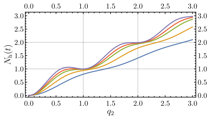
FIG. 4. Total number of injected holes as a function of q_2 = q \cos \theta \sin \theta at zero temperature, in the case of a Lorentzian drive. Different curves refer to (from bottom to top) t/w = 5, 10, 20, 30, 50 . The ratio between slow and fast velocities is \gamma = 1/5 .
