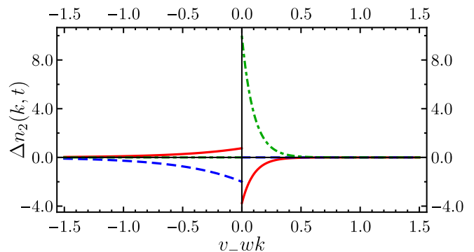
FIG. 3. Overlap distribution (33), together with stationary ones (27), in the case q_2 = 1 . The blue (green) dashed (dot-dashed) line represents \Delta n_{2-} ( \Delta n_{2+} ), while the red full line is 20\Delta n_{2X} for t/w = 8 . Note that the latter describes electron (hole) excitations for negative (positive) momenta, in contrast with the behavior of the stationary distributions (27). In this plot we have used \gamma = 1/5 .
