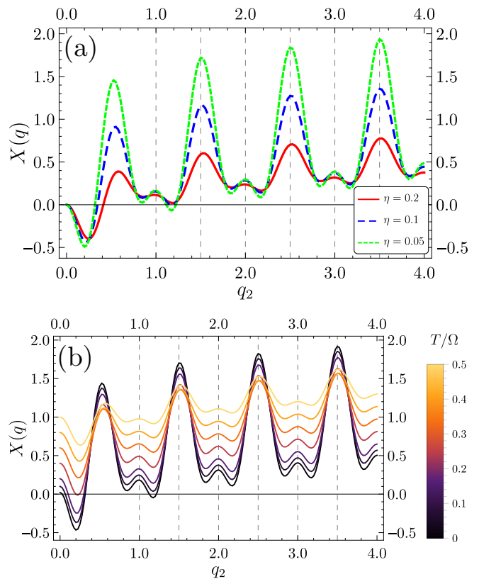
FIG. 7. The quantity X , defined in (46), as a function of q_2 for a rectangular pulse. (a) Zero-temperature result for different values of \eta . Principal maxima are very well located at half-integer q_2 already for \eta = 0.1 . In addition, the smaller \eta the bigger the amplitude of oscillations. (b) Different curves for temperatures ranging from zero to T = \Omega/2 and \eta = 0.05 . In both panels the time delay is \tau_d = \mathcal{T}/2 .
