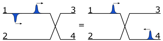
FIG. 5. Equivalence between the investigated HBT setup at \nu = 2 (left) and a non-interacting HOM setup at \nu = 1 (right). In the first one, the two oppositely-charged excitations on the inner channel arrive at a QPC from the left side and are separated due to the fractionalization phenomena. In the second one, two excitations with the same charge arrive at a QPC from opposite sides and are separated due to the time delay between the drive applied at terminal 1 and the one at terminal 4.
