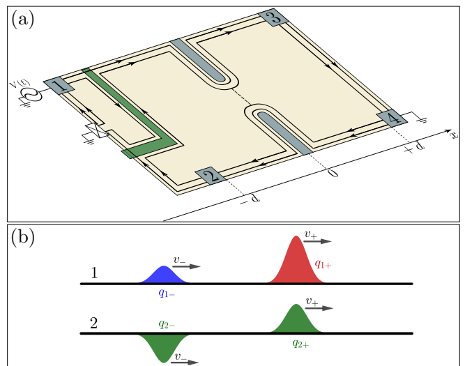
FIG. 1. (a) Sketch of the considered setup. A time-dependent external voltage drive applied at terminal 1 drives the system out of equilibrium, exciting electron wave packets into the edge channels. Right after the driven contact, a gate (green) acts as a filter, transmitting only outer-channel excitations. After a propagation distance d , a quantum point contact is set to fully transmit the outer channel and partially reflect the inner one, thus creating current fluctuations at terminals 2 and 3 (see Sec. IV). (b) Sketch of the fractionalization of the excited pulse: for q > 0 [see Eq. (15)] two electron-like excitations are created in the outer channel, while hole-like ( q_{2-} ) and electron-like ( q_{2+} ) excitations emerge in the inner channel, to which it is not transferred any net charge.
