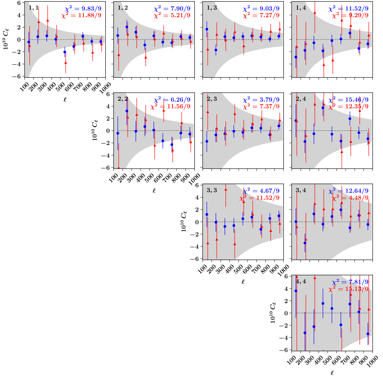
Figure 24. The measured B-mode in METACALIBRATION (blue circles) and IM3SHAPE (red triangles), and the corresponding detection \chi^2 values. The measurements use the tomographic bins 1 to 4 as used in Troxel et al. (2017), and the auto- and cross-correlations between them are shown. The value is expected to be close to zero in the absence of systematics. Error bars were calculated from a set of log-normal simulations matching the DES-Y1 survey geometry and redshift distributions. The grey band show \pm the E-mode signal in a fiducial cosmology.
