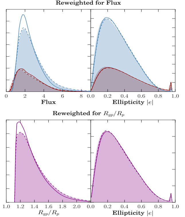
Figure B1. Histograms of flux (upper left), size (lower left) and ellipticity (upper/lower right) in the data (shaded region) and simulations used for IM3SHAPE calibration before (solid) and after (dashed) objects are reweighted to match the flux (top) and size (bottom) distributions in the data. In the upper panel we show bulge and disc galaxies separately in red and blue respectively.
