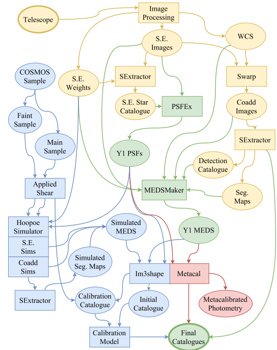
Figure 1. A flow-chart showing the steps in the DES Year 1 shape analysis, starting from low-level calibrated data products made by DES Data Management (DES-DM) and ending with final output catalogues. Yellow stages are performed in the DES-DM software process. Green stages are performed in the Weak Lensing analysis process. Blue stages are part of the IM3SHAPE process, mostly simulation and calibration, and red stages part of the METACALIBRATION analysis. “S.E.” stands for “single epoch”.
