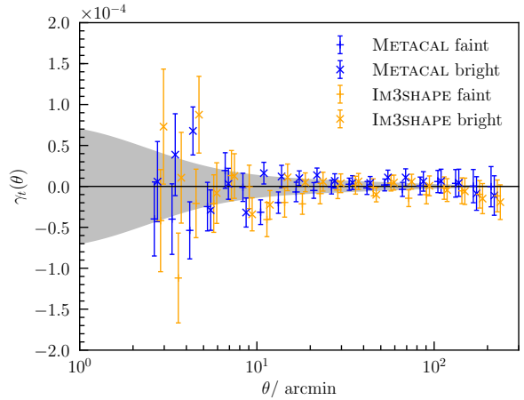
Figure 21. Tangential shear around stars, which have been split into a bright ( 14 < m_i < 18.3 ) and a faint sample ( 18.3 < m_i < 22 ). The faint sample includes stars used for PSF modelling while bright stars are used to test other effects related to the saturation around them. The error bars come from the jackknife method. The grey band is 10% of the weakest expected signal, as in Figure 17. The deviations from null in this test at small scales were excluded by the scale cut \theta > 30 arcmin.
