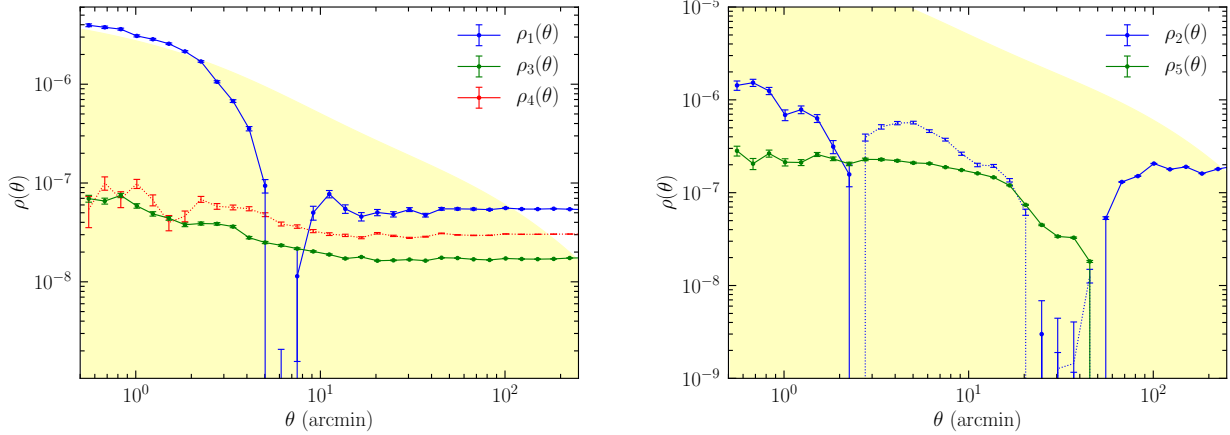
Figure 9. The \rho statistics for the PSF shape residuals. Negative values are shown in absolute value as dotted lines. Requirements on the \rho statistics are specific to individual science cases; the yellow fill is a general guide, rather than a requirement, and is ten percent of the value of the weakest cosmic shear \xi_+ signal, which is from the lowest redshift tomographic bin (for this bin only scales above \theta \approx 7 arcmin were used in the analyses in Troxel et al. 2017 and DES Collaboration 2017). It pessimistically assumes \alpha = 0.1 and T_{\text{PSF}}/T_{\text{gal}} = 1 . Contributions to the signal from the flat regimes at large scales will be absorbed by the marginalization over the mean shear discussed in §7.1.
