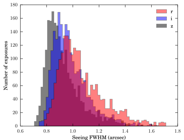
Figure 6. The distribution of the median seeing FWHM of the stars used to model the PSF in the riz -bands. The median seeing of these distributions is 1''.03 in the r -band, 0''.95 in the i -band, 0''.89 in the z -band, and 0''.96 in the three bands overall.
