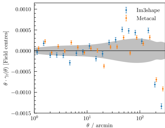
Figure 17. The tangential shear of galaxies in the two catalogues around field centres, after subtraction of shear around random points. The grey band shows ten percent of the weakest tangential shear signal around galaxies in any of the galaxy-galaxy lensing measurements used in Prat et al. (2017) . This weakest signal combination was from lens bin 3, source bin 4; the data from this combination were used only at \theta > 30 arcmin. As noted in the text the deviations from nullity are significant, and a further test was done to ensure that they did not impact our galaxy-galaxy lensing science.
