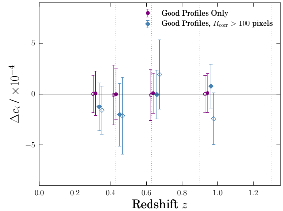
Figure A2. Change in the multiplicative bias (top) and additive bias (bottom) after removal of bad COSMOS profiles, relative to the value derived using all galaxies. In the lower panel the filled markers show the c_1 component and the open ones show c_2 .
