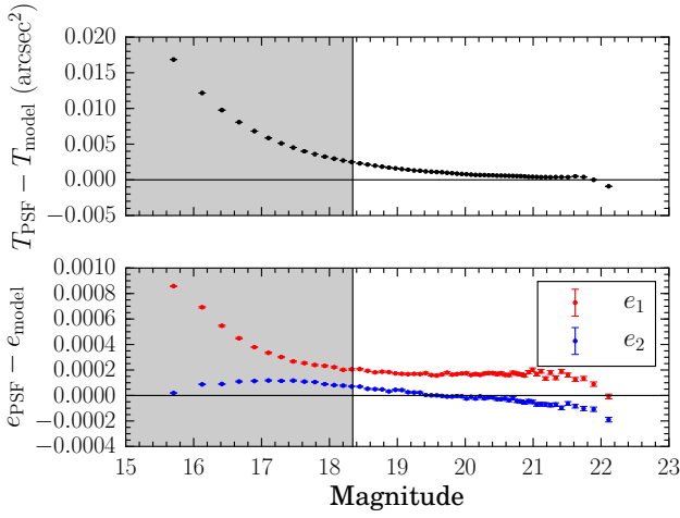
Figure 7. The relative model size (top) and shape (bottom) residual of stars. To reduce the impact of the brighter-fatter effect bright stars are excluded from our PSF models; the cut-off varies between CCD exposures but the shaded region shows a typical example.
