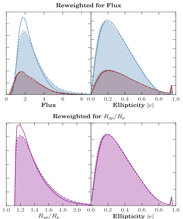
Figure B1. Histograms of flux (upper left), size (lower left) and ellipticity (upper/lower right) in the data (shaded region) and simulations used for IM3SHAPE calibration before (solid) and after (dashed) objects are reweighted to match the flux (top) and size (bottom) distributions in the data. In the upper panel we show bulge and disc galaxies separately in red and blue respectively.
