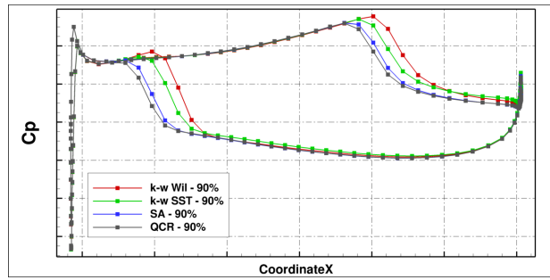
(b) Fan blade pressures with URANS simulation, 90% height.
