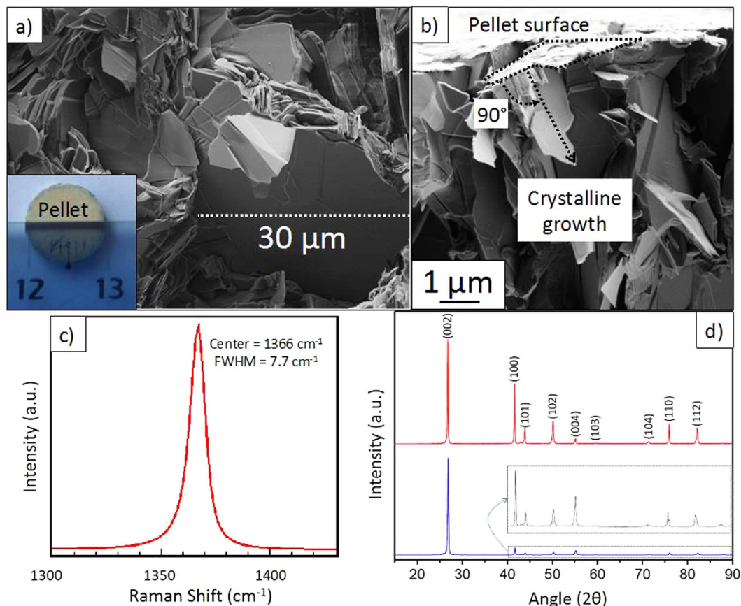
Figure 1. (a) SEM image showing stacked layers with micrometric sizes, inset: 1 cm-diameter pellet; (b) SEM image showing the pellet cross section and BNNs aligned perpendicularly to the surface pellet; (c) Raman scattering spectrum recorded on the raw sample and (d) XRD patterns obtained with the raw sample (upper) analysis of the pellet surface and (bottom) analysis of the pellet cross-section.
