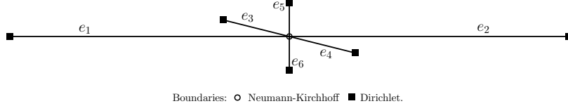
Figure 8: Example of star graph described by Theorem 4.3 with N = 6 .
