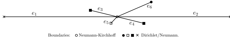
Figure 4: Example of graph described in Corollary 3.4 with \tilde{N} = 4 and N = 6 .
