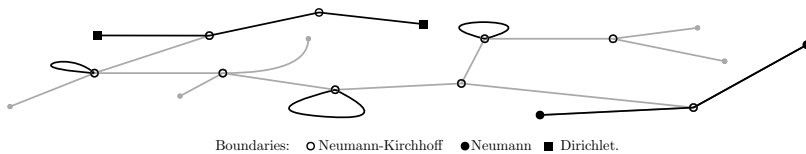
Figure 6: The figure underlines the uniform chains in a generic compact graph.
