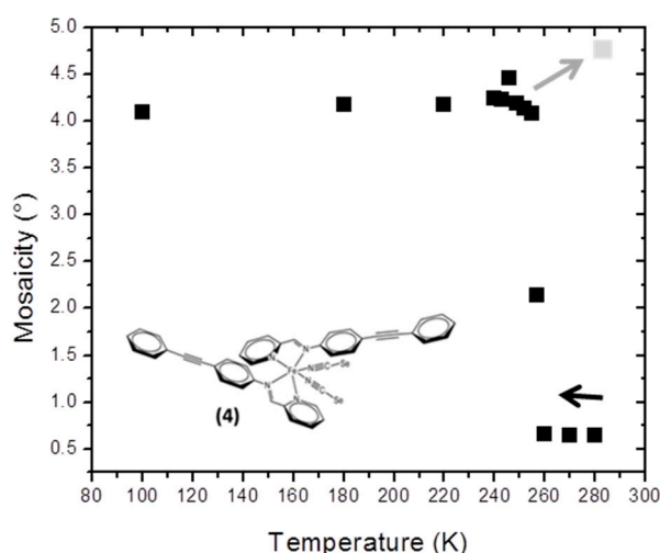
Figure 4. Temperature dependence of the mosaicity of [Fe(PM-PeA)_2(NCSe)_2] in the cooling mode (black squares), including the return values (light grey) after warming at room temperature.
