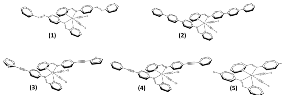
Scheme 1. schematic views of the molecular iron(II) complexes of the [\text{Fe}^{\text{II}}(\text{PM-L})_2(\text{NCX})_2] series studied in this paper, labelled 1 to 5.
