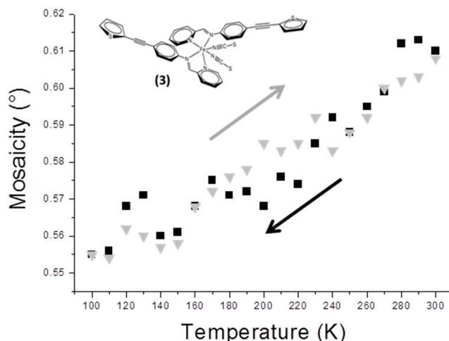
Figure 3. Temperature dependence of the mosaicity for a crystal of [Fe(PM-TheA)_2(NCS)_2]-II in the cooling (black squares) and warming (light-grey triangles) modes.
