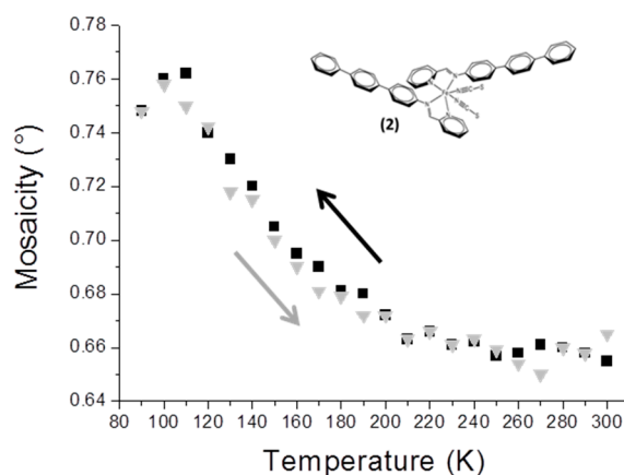
Figure 2. Temperature dependence of the mosaicity for a crystal of [\text{Fe}(\text{PM-TeA})_2(\text{NCS})_2] \cdot 0.5\text{MeOH} in the cooling (black squares) and warming (grey triangles) modes.
