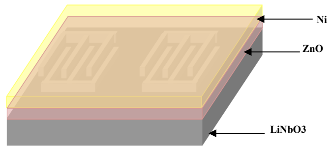
Fig. 5: Schematic view of a Ni/ZnO/IDT/LiNbO 3 SAW structure.
