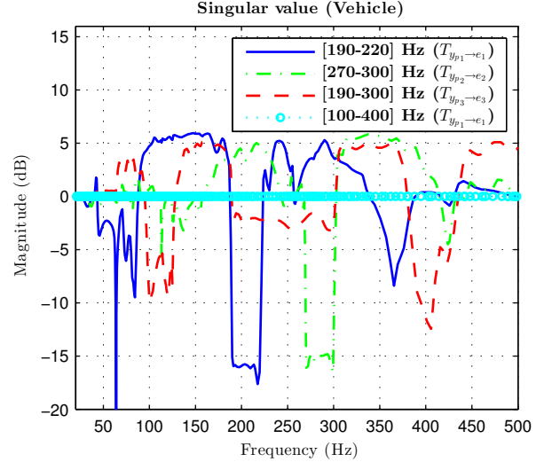
Figure 13: Magnitude of the transfer associated with the criterion value of Table 6 (Vehicle, Simulation)
