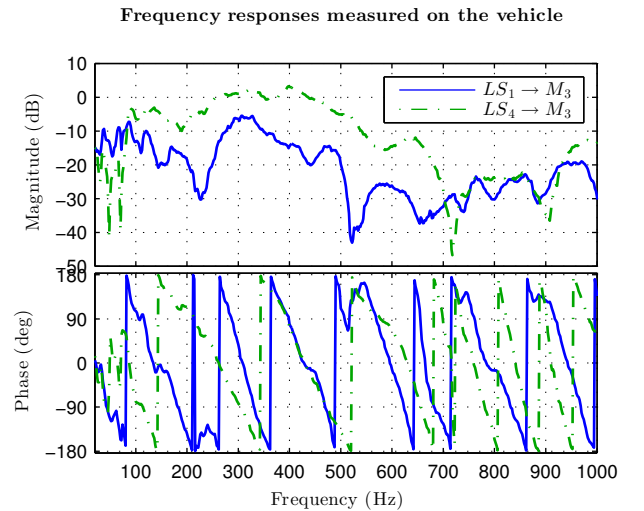
Figure 2: Frequency responses measured on the vehicle
