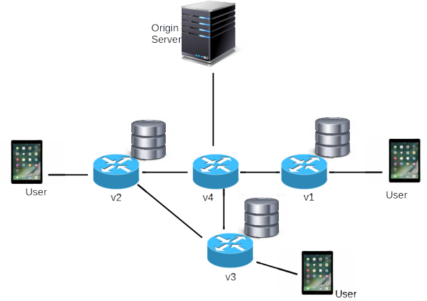
Figure 1: An example of Content-based Centrality (Closeness)
