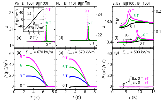
FIG. 3. A -cation controlled magnetoelectric properties in the A(\text{TiO})\text{Cu}_4(\text{PO}_4)_4 system. Temperature ( T ) dependence of (a) the dielectric constant along the [100] direction \varepsilon_{[100]} and (b) electric polarization P_{[100]} for the Pb system in various magnetic fields applied along the [100] direction ( B_{[100]} ). (c) Isothermal P_{[100]} - B_{[100]} curve at 2.5 K. T dependence of (d) \varepsilon_{[110]} and (e) P_{[110]} in various strengths of B_{[110]} for the Pb system. T dependence of (f) \varepsilon_{[100]} and (g) P_{[100]} in various strengths of B_{[110]} for the Ba and Sr systems. In (b), (c), (e), (g), the values of electric field applied during ME cooling ( E_{\text{cool}} ) are indicated.
