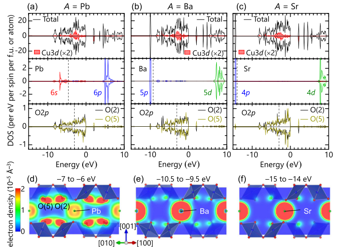
FIG. 4. Total DOS and Cu 3 d , A site, and O 2 p partial DOS of A = (a) Pb, (b) Ba, and (c) Sr systems. The Cu 3 d partial DOS is multiplied by 2 for clarity. The dashed vertical lines indicate the band center of mass (see text). Real-space electron density map for A = (d) Pb, (e) Ba, and (f) Sr systems in the energy window where the A partial DOS is large. The color represents the magnitude of electron density.
