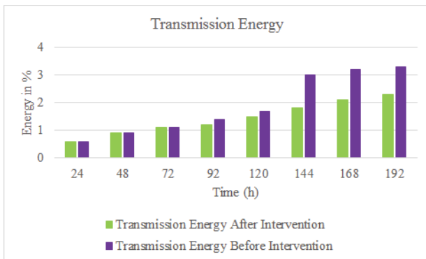
Fig. 10. Transmission Energy
