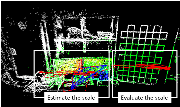
Figure 15: Evaluation of the estimated scale. The reconstructed environment includes a calibration board. First, estimate the scale of the point cloud. Second, compare the estimated scale and the actual scale by using the side of the calibration board.
