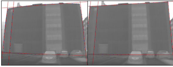
Figure 4: Estimation of distortion parameter. (Left) A set of points supposed to be aligned in the real scene and their least-square fitted line. (Right) Corresponding undistorted image.
