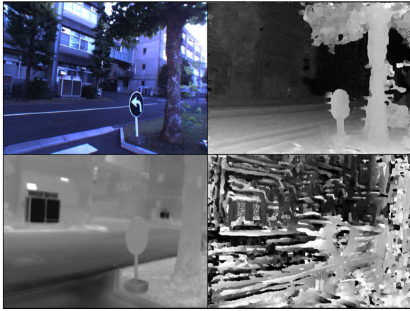
Figure 9: Generating a depth map using a multi-view stereo (MVS) algorithm. The top left shows a reference RGB camera image and the bottom left shows a reference thermal-infrared camera image. Right images show the result of MVS using each image.
