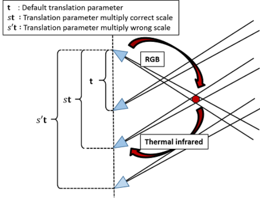
Figure 7: Variation of back-projection by different scale. The red circle represent a 3D object of the scene, with a certain arbitrary scale. The translation \mathbf{t} between the two cameras is initially subject to \|\mathbf{t}_{ir}\|^2 = 1 can be scaled with the fine scale factor s to fit the 3D reconstruction from the first camera.
