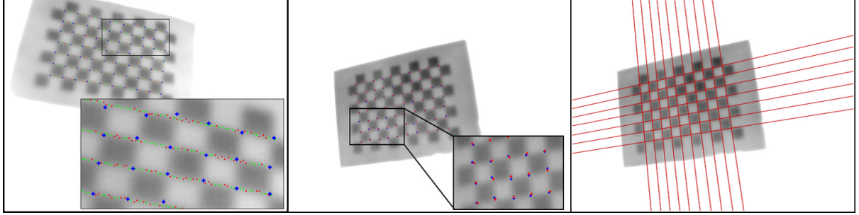
Figure 5: Initial detection and refining the points. Refined corner points should lie along straight lines in the left image. The center image shows the refinement of the points. Blue points are points detected by OpenCV and Red Points are the refined points, and the right image shows lines drawn connecting the corners.
