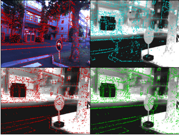
Figure 8: Result of back-projection to thermal-infrared images using different scales. The top left is a reference RGB camera image. The other images are generated by back-projection of the DSO point cloud using different scales. The bottom left image shows the accurate scale.
