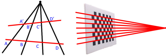
Figure 6: Constraints of cost function. The left figure describes the cross-ratio constraint, which is satisfied by Eq. (2). The right figure shows vanishing point of the calibration board.
