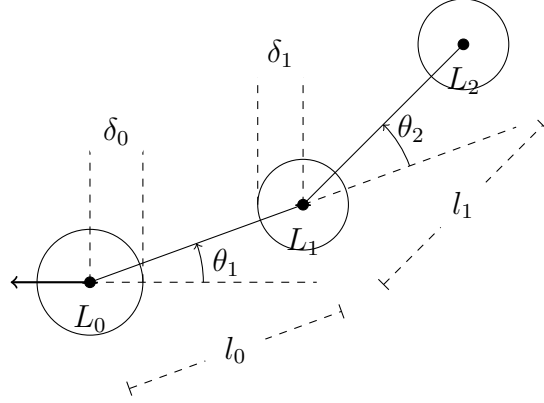
Figure 8: N = 2 serial kinematic chain system
