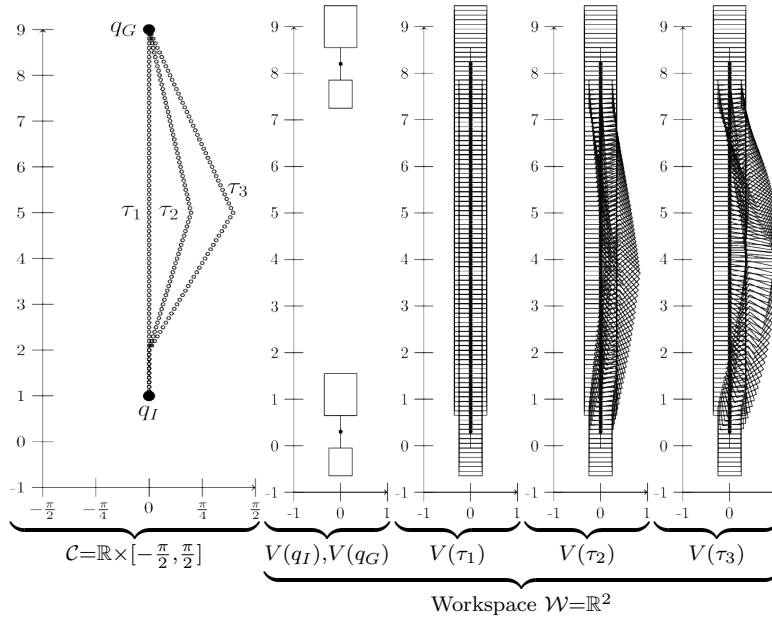
Figure 2: Explanatory example of irreducible paths for a 2-link, 2-dof robot, which can move along the y -axis, and which has one rotational joint between its two links, such that its configuration space is \mathcal{C} = \mathbb{R} \times [-\frac{\pi}{2}, \frac{\pi}{2}] . Left. Three configuration space paths \tau_1, \tau_2, \tau_3 with \tau_1(0) = \tau_2(0) = \tau_3(0) = q_I , \tau_1(1) = \tau_2(1) = \tau_3(1) = q_G . Right. The workspace volume of the starting configurations q_I, q_G , and the swept volume of the three paths, whereby we have that V(\tau_1) \subset V(\tau_2) and V(\tau_1) \subset V(\tau_3) , i.e. \tau_2 and \tau_3 are reducible by \tau_1 , and \tau_1 is in fact irreducible. Adapted from [6].
