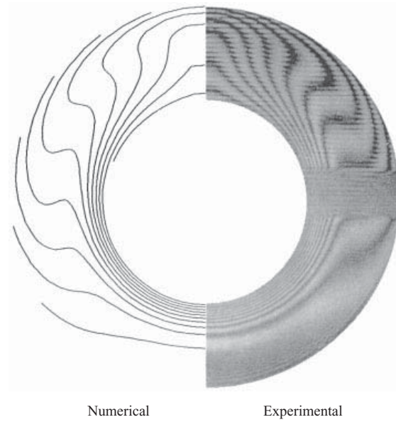
FIGURE 19. Comparison of isotherms at the mid-axial plane for Ra = 1.1 \times 10^4 , R = 2.18 , Pr = 0.7 .
