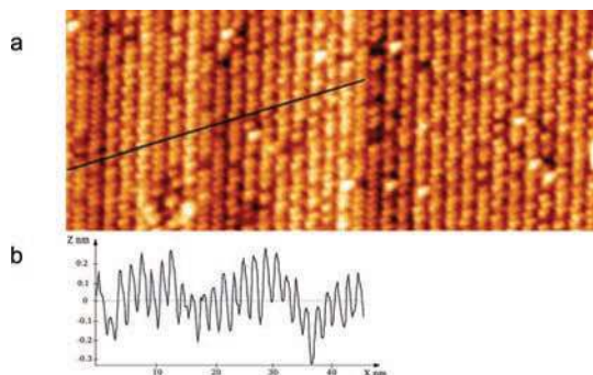
Figure 4. (a) Large scale STM image ( 60 \times 25 \text{ nm}^2 , V_s = -1.7 \text{ V} and I = 0.6 \text{ nA} ) of the nanolines network on Si(111)-B \sqrt{3} \times \sqrt{3} \text{ R}30^\circ surface at room temperature and (b) z -profile along the dark line.
