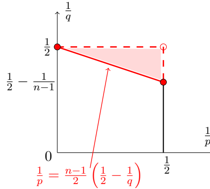
FIGURE 2. Admissibility in dimension n \geq 4 .
