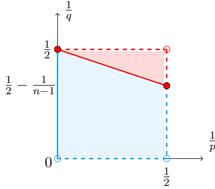
FIGURE 3. Case n \geq 4
