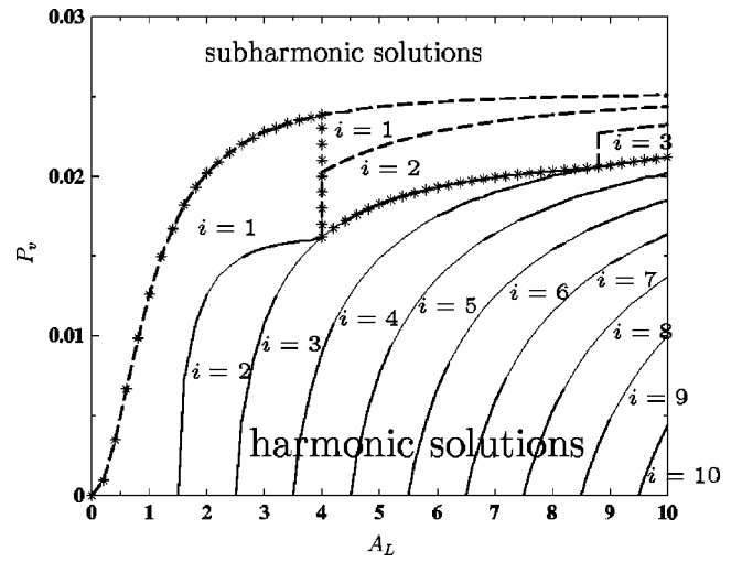
FIG. 3. For a chosen pair (A_L - P_v) , the figure indicates the number i of cells on the emerging branch of the synchronous solution. For a fixed A_L value, the crossover values of P_v between the synchronous and subharmonic solutions are given by the stars. For all P_v under the stars, the first primary bifurcation gives rise to synchronous solutions.
