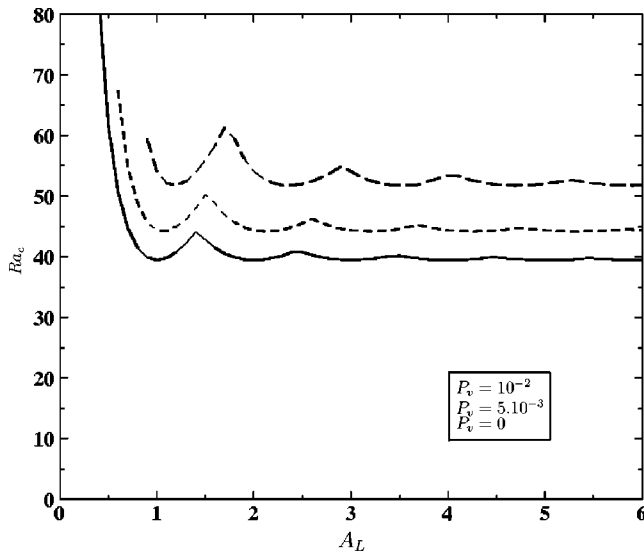
FIG. 1. Critical Rayleigh number Ra_c of the first primary bifurcation point is the aspect ratio A_L . In the Ra_v formulation, Ra_c \rightarrow \infty when Ra_v \rightarrow \infty , Bardan and Mojtabi (Ref. 10). In the P_v formulation, there exists a limit value P_{v_l} which cannot be exceeded.
