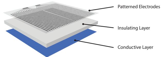
Figure 8. A ShapeMe grid of sensors consists of a layer of patterned electrodes (inkjet printed), a common back electrode (screen-printed), and an insulating layer between them.
