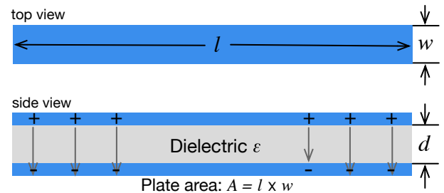
Figure 5. Schematic depiction of a parallel-plate capacitor.
