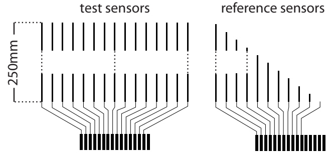
Figure 10. Configuration of sensors on our experimental sheets
