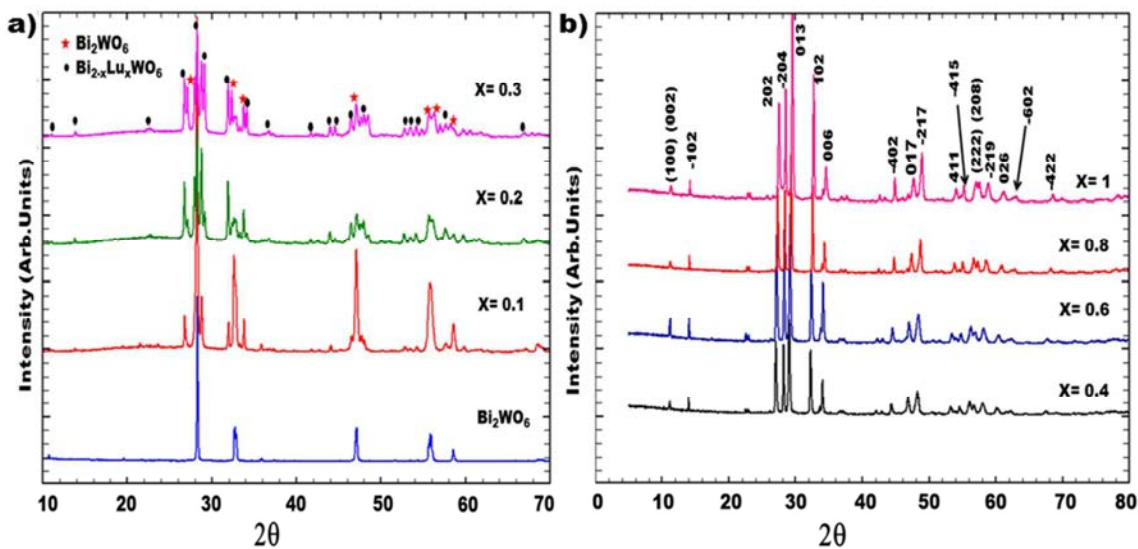
Figure 1: XRD pattern of the \text{Bi}_{(2-x)}\text{Lu}_x\text{WO}_6 obtained in room conditions : a) Biphasic system up to x=0.3 ; b) monoclinic solid solution up to x=1 .
