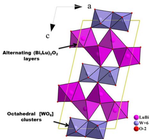
Figure 6: Crystal structure of monoclinic \text{Bi}_{2-x}\text{Lu}_x\text{WO}_6 compounds in the (010) plane.
