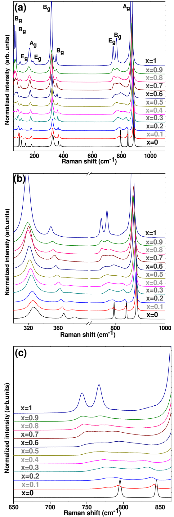
Fig. 5. (a) Room temperature Raman spectra of Sr 1-x Pb x MoO 4 , for 0 \leq x \leq 1 , (b) Zoom in the number wave domain 325–1000 cm -1 (c) Zoom in of the Eg and Bg modes ( \lambda (excit.) = 514.5 nm).
