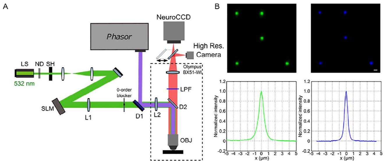
Figure 1. Two-colour CGH illumination: A) Diagram of the optical setup for holographic illumination patterns at 532 nm and 405nm. The 532 nm (green) laser beam from a solid-state laser is attenuated by neutral density filters (ND), enlarged by a telescope, and directed to the liquid crystal SLM. The plane of the SLM is projected with an afocal telescope (L1 and L2) to the back aperture of a microscope objective (OBJ). The 405 nm patterned beam (violet) is generated by a commercial module (Phasor) and coupled to the 532 nm beam path through a dichroic mirror D1. The patterned beams are reflected toward the objective by the dichroic mirror D2. The collected fluorescence is filtered by the long pass filter (LPF) and directed either to high resolution camera or to the high-speed NeuroCCD camera using a movable mirror. B) Upper panels: Fluorescence pattern generated by a 532 nm (right) and 405 nm (left) digital holography on a thin layer of Rhodamine 6G as detected with the NeuroCCD. These patterns were used to calibrate the sub-micrometric positioning of the holographic spots. Scale bar 1 \mu\text{m} . Lower panels: Spatial profile of the Rhodamine emission generated by a 532 nm (green) or 405 nm (blue) CGH spot recorded with the high resolution camera.
