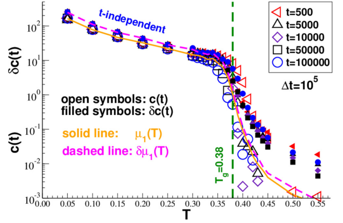
FIG. 19. Ensemble-averaged ACF c(t) (open symbols) and associated standard deviation \delta c(t) (filled symbols) as a function of temperature T for several times t . Note that \delta c(t) is always larger c(t) for all T and t . The bold solid line indicates \mu_1(T) for \Delta t = 10^5 , the dashed line the corresponding standard deviation \delta\mu_1(T) . Below T_g , one observes c(t) \approx \mu_1(T) and \delta c(t) \approx \delta\mu_1(T) .
