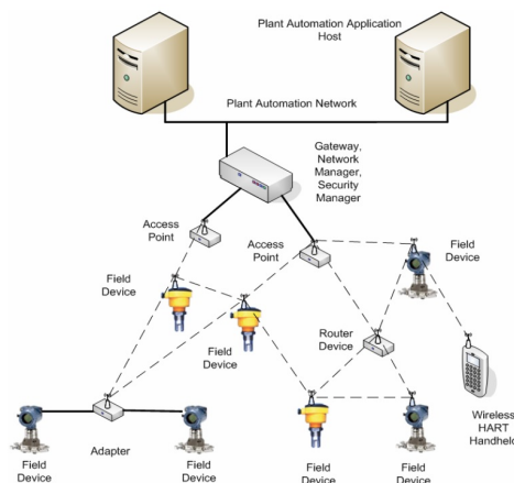
Fig. 1. Example of a WirelessHART network [10]
