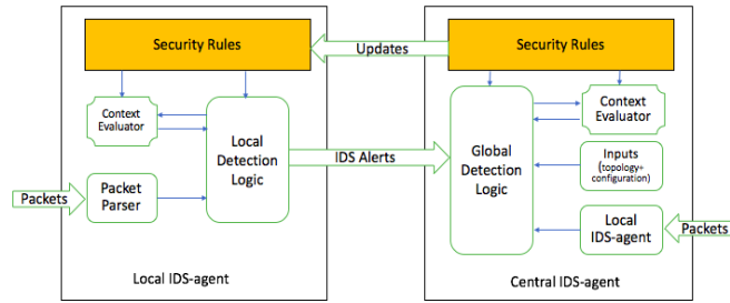
Fig. 2. The Central-IDS and IDS-Agents Architecture
