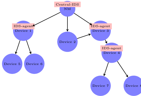
Fig. 3. IDS-agents deployment
