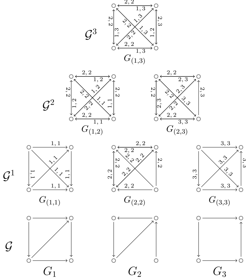
Fig. 8: Example of a round trip transitive closure hierarchy of a dynamic graph \mathcal{G} of length \delta = 3 . (Arrival and departure times are on the head ends of the arrows.)
